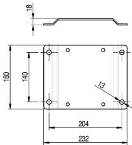
FIXING BRACKET
